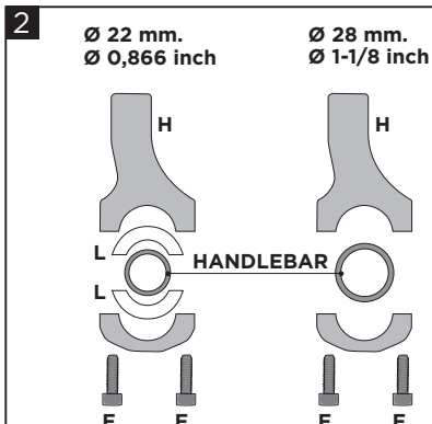
H - (2 PCS)
